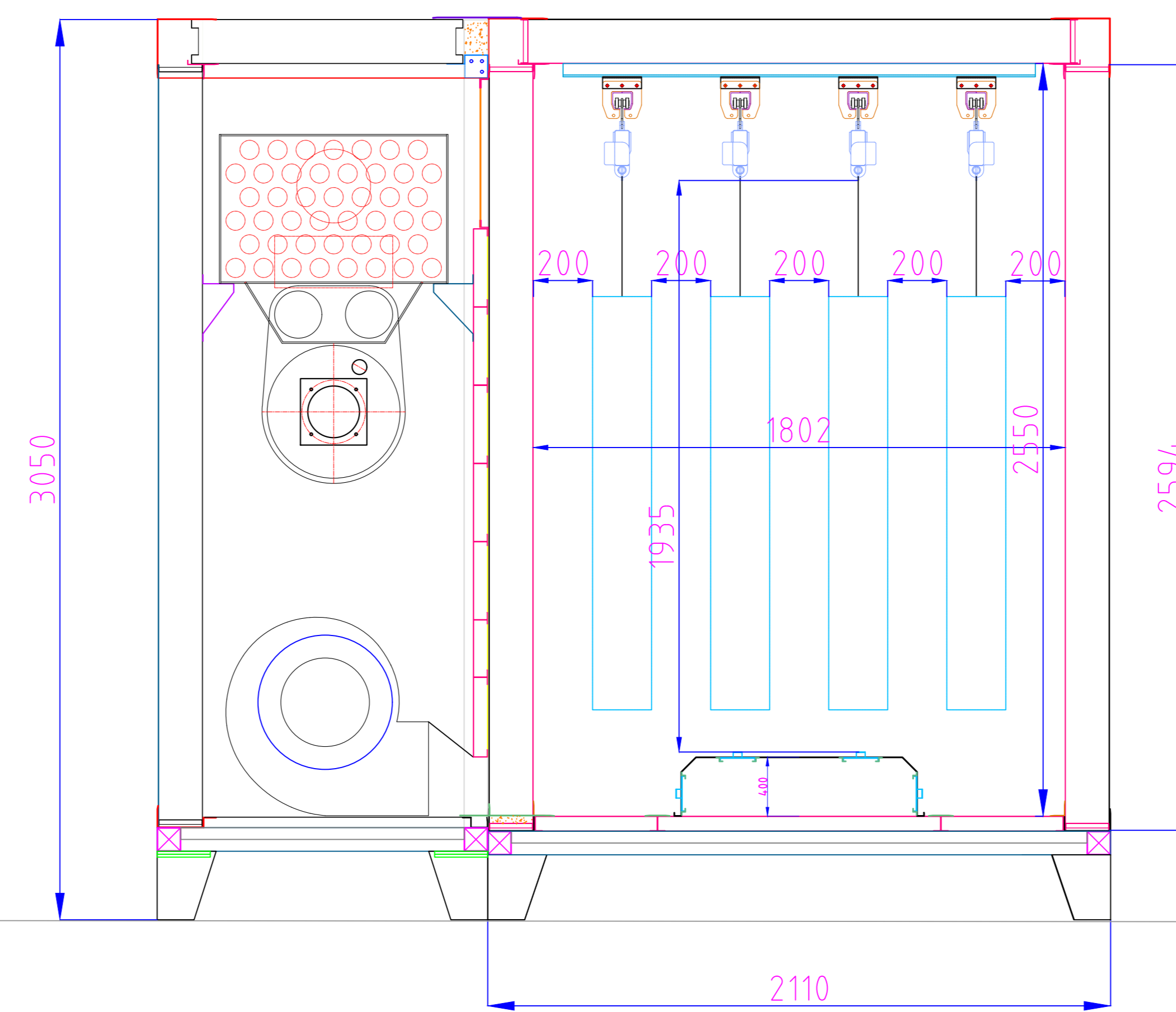
PF-5 CURING OVEN SCALE : 2:1
