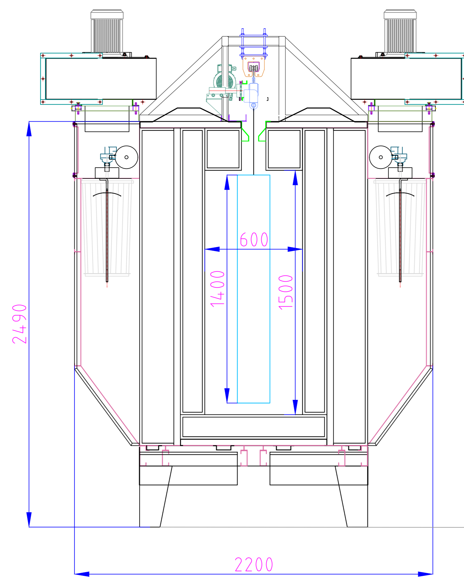
FK-8 POWDER BOOTH SCALE : 2:1
